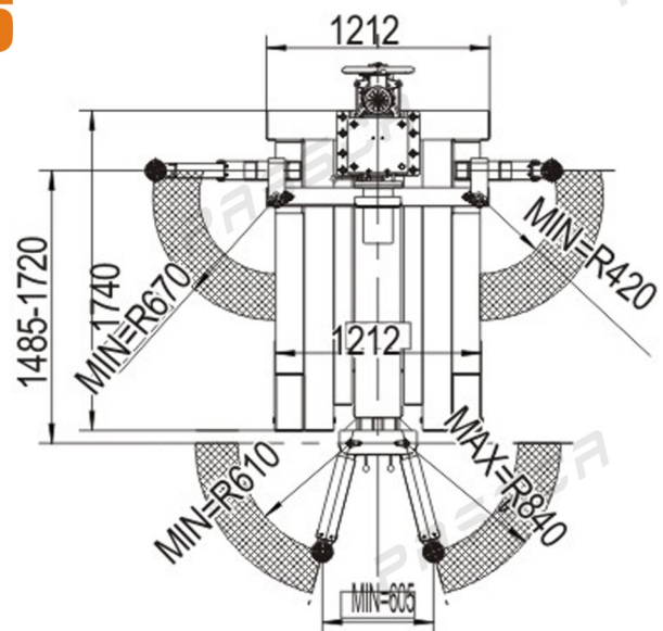
Mobile Single Post Lift, Manual Lock Release
