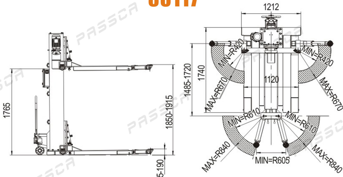
Mobile Single Post Lift, Automatic Lock Release
