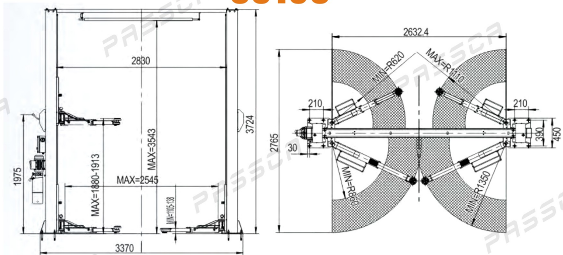
Electro-Hydraulic 2 Post Lift Clear Floor Plate Type, Manual Single Side Lock Release
